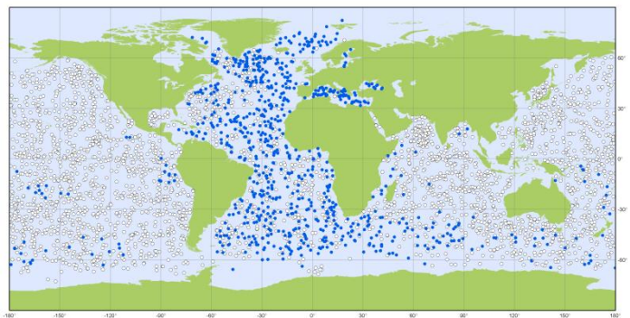
Argo European contribution to the Argo program via EuroArgo Research Infrastructure Latest locations of operational profiling floats (date distributed within the last 30 days) May 2018
